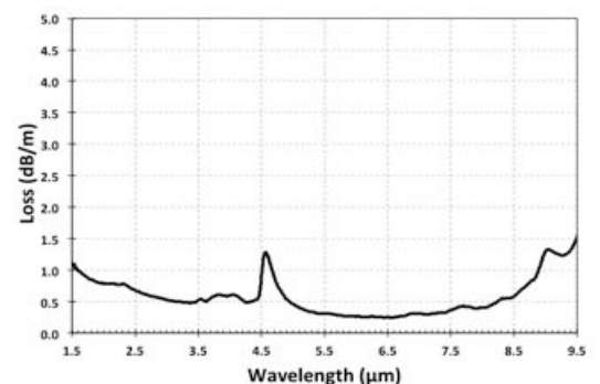
Attenuation Spectrum for IRF-Se series
