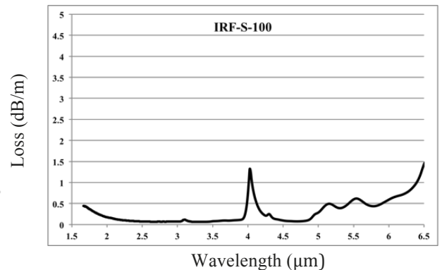
IRF-S-100 Attenuation Spectrum
